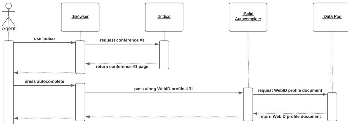
Fig. 17: Sequence diagram showing the sequential process through pulling in data from a data pod.
